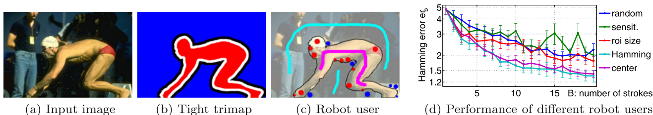
Fig. 2 An image from the database (a), tight trimap (b), robot user ( red/blue ) started from user scribbles ( magenta/cyan ) with segmentation ( black ) after B = 20 strokes with 1.4 % error (c) and performance comparison of different robot users (d)
